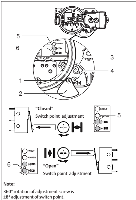
Fig. 5.3 Re-adjustment screws for "Open" and "Closed" position feedback
