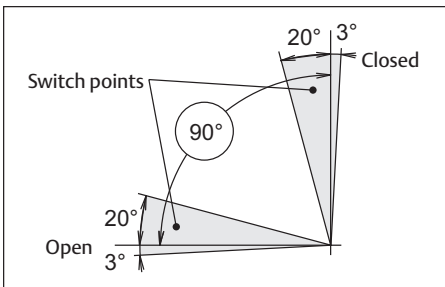
Fig. 5.1 Adjustable range
