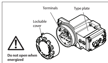
Fig 11.1 Product marking
