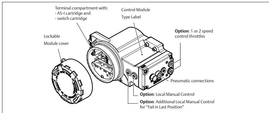
Fig 2.4 Control module overview
