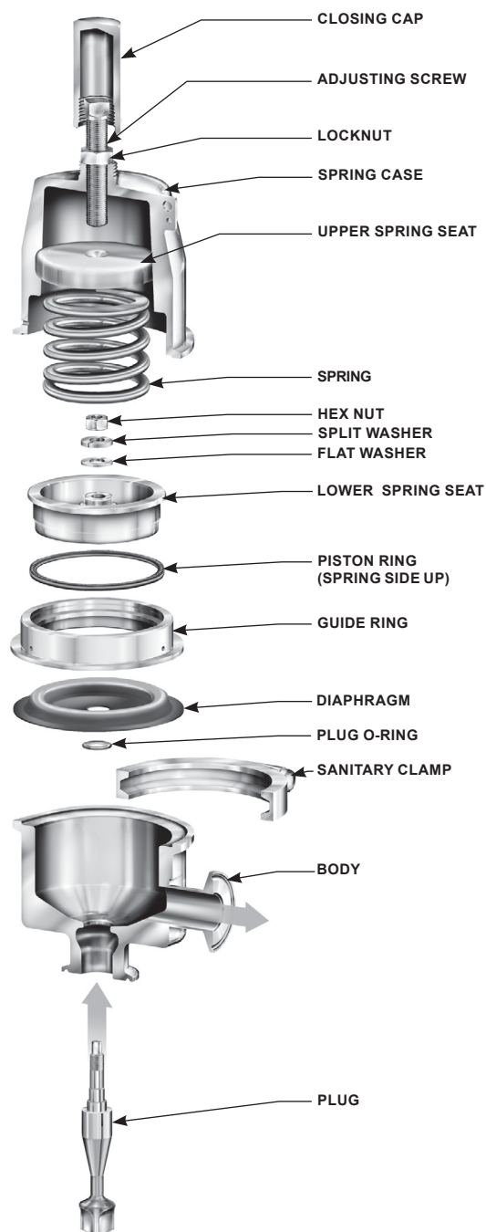
Figure 3. Type SR5 Parts Explosion
