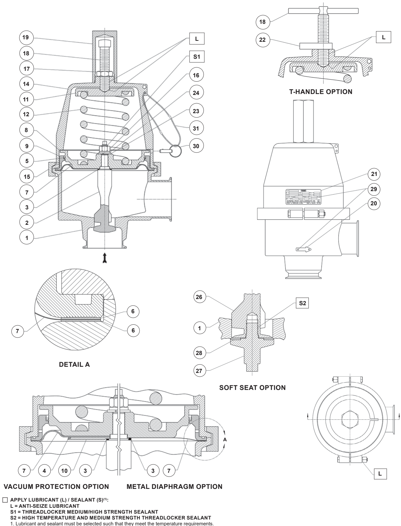
Figure 6. Type SR5 Sanitary Regulator Assembly 2 and 3 In. / 50 and 80 mm Sizes
