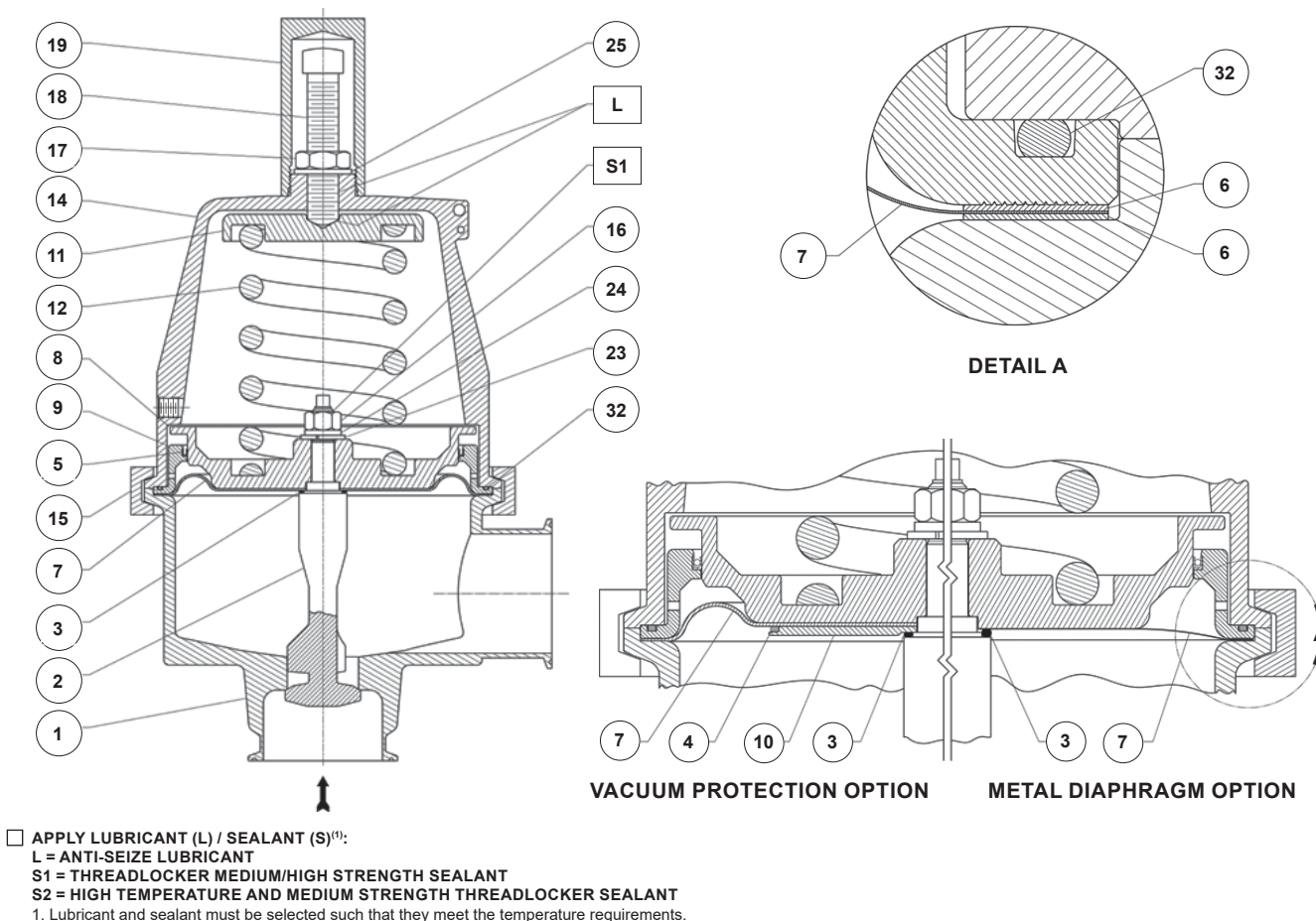
Figure 7. Type SR5 Sanitary Regulator Assembly with Pressure Loaded Spring Case 2 and 3 In. / 50 and 80 mm Sizes
