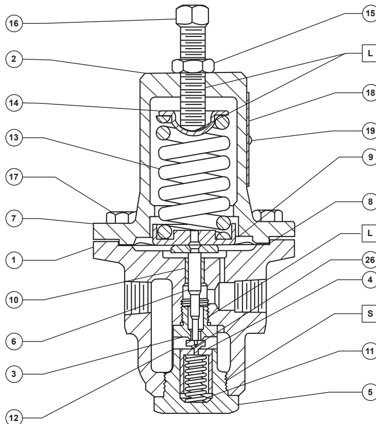
Figure 8. Type 92C Steam Regulator Assembly
