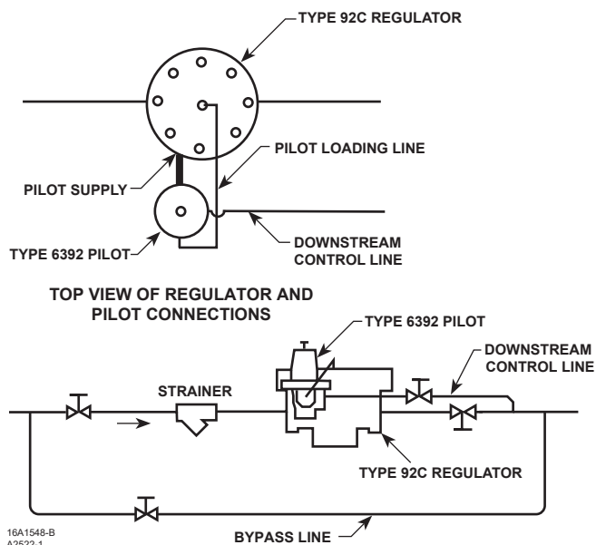
Figure 3. Typical Pilot-Operated Type 92C Regulator Installation
