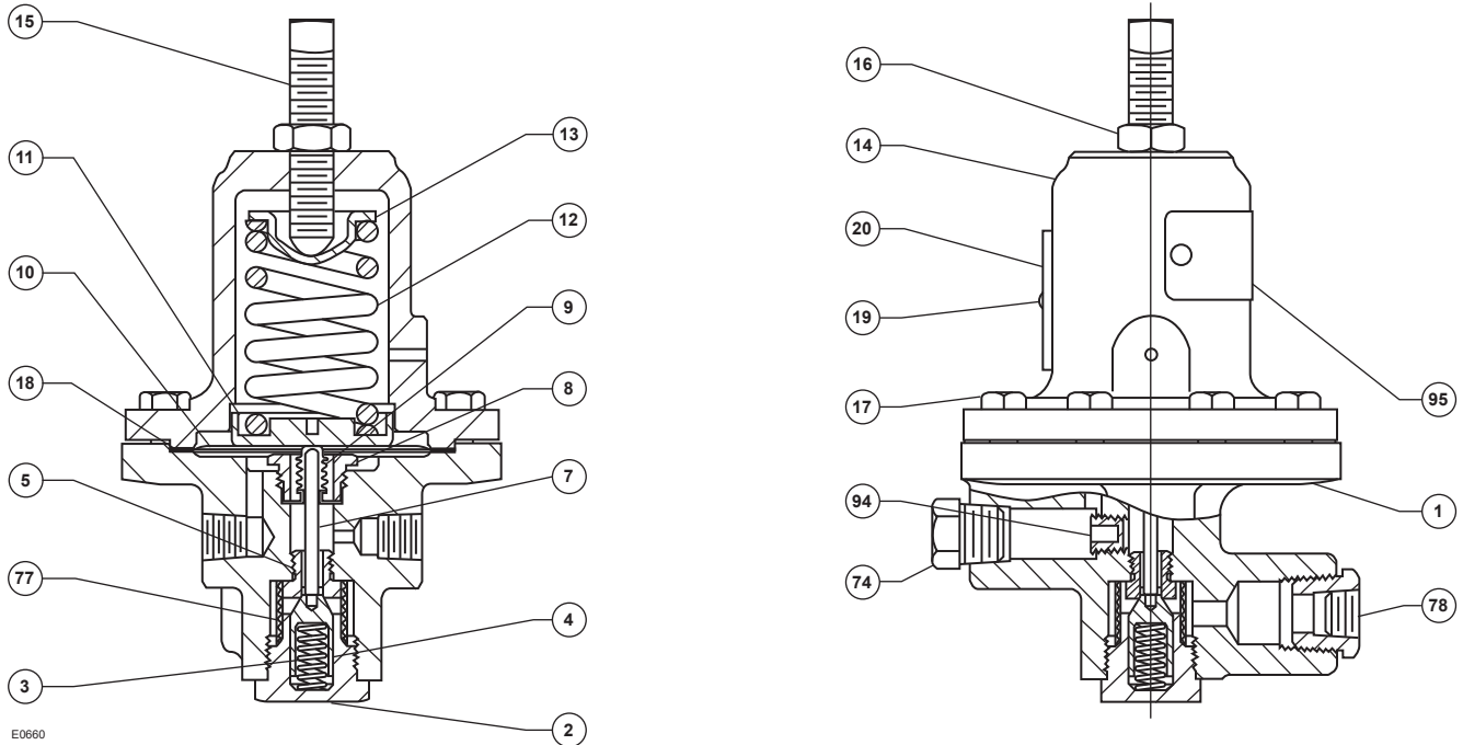
Figure 11. Type 6492HM or 6492HTM Safety Override Pilot Assembly
