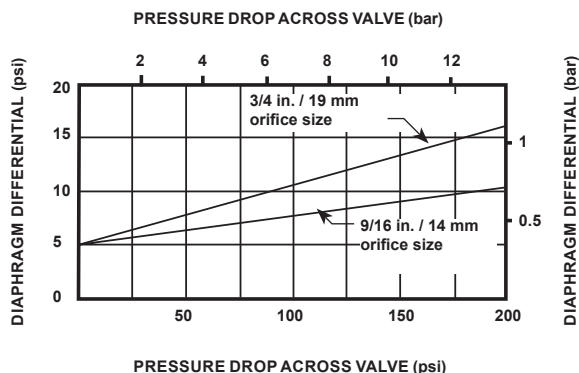
Figure 2. Diaphragm Differential Pressure for Pressure-Loaded Regulator
