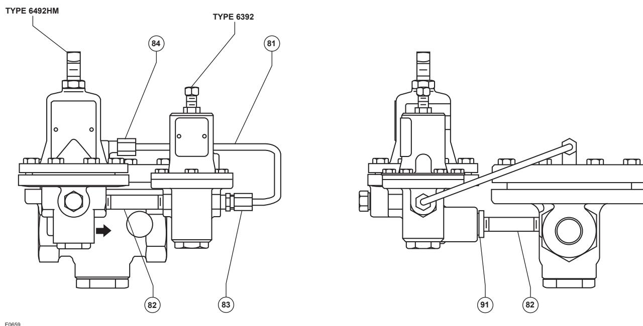
Figure 12. Type 92C with Safety Override Pilot Assembly
