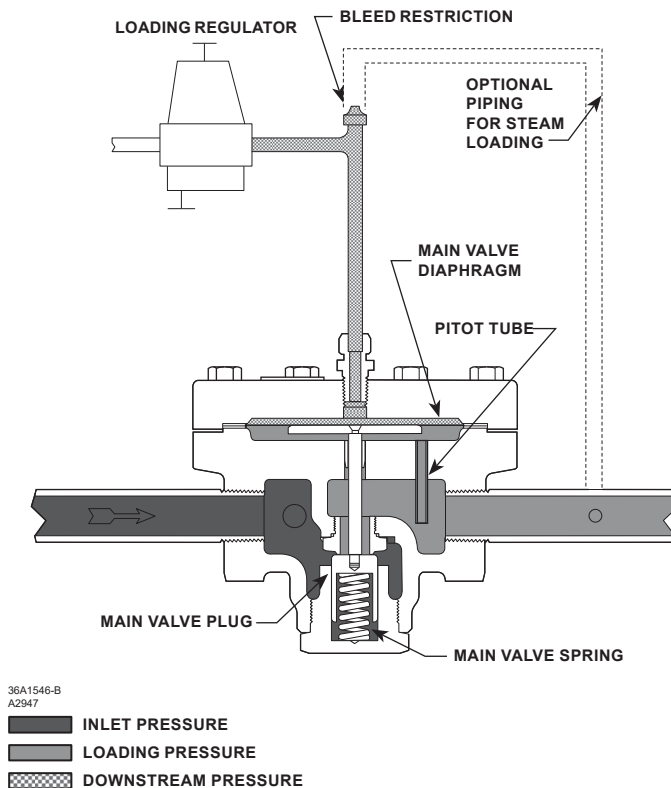
Figure 7. Operational Schematic of Pressure-Loaded Type 92C Regulator
