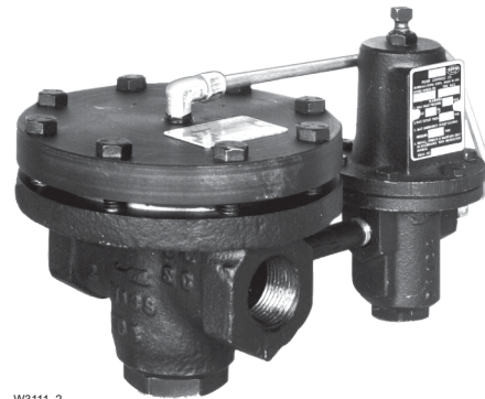
Figure 1. Type 92C Pilot-Operated Regulator
